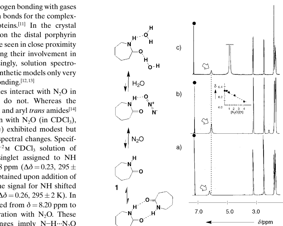
Figure 1. Complexation-induced changes in the 1 H NMR spectrum (500 MHz, CDCl 3 , 295 ± 2 K) of \epsilon -caprolactam 1 : a) solution of 1 , 5 × 10 −2 M; b) same, after saturation with N 2 O; c) same, after saturation with H 2 O. In two independent experiments, saturation of both 1 and 1 :N 2 O solutions with H 2 O gave identical spectra. An arrow marks the NH signal. The residual CHCl 3 signal is marked ●.
